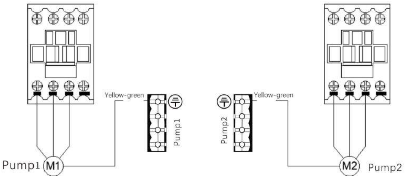
Three-phase motor connection
