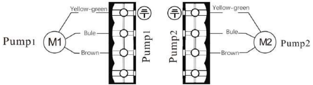
Wiring of single-phase motor with built-in capacitor
