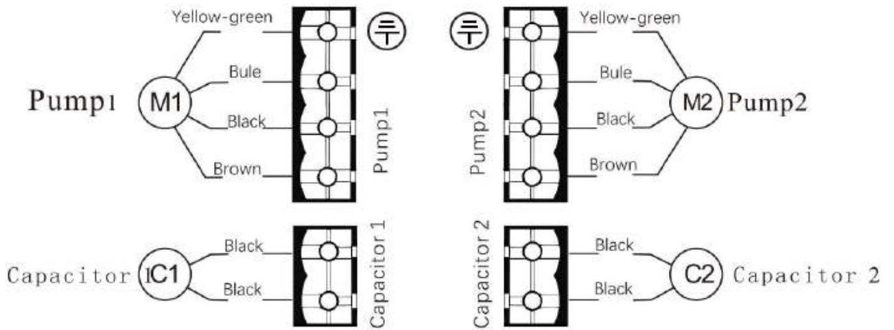
Wiring of single-phase motor with built-in capacitor
