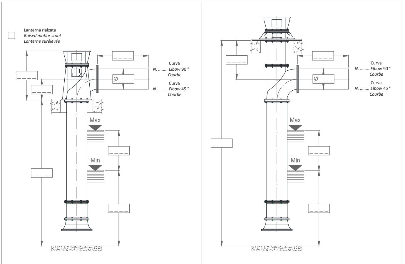
Installazione standard Standard installation Installation standard
