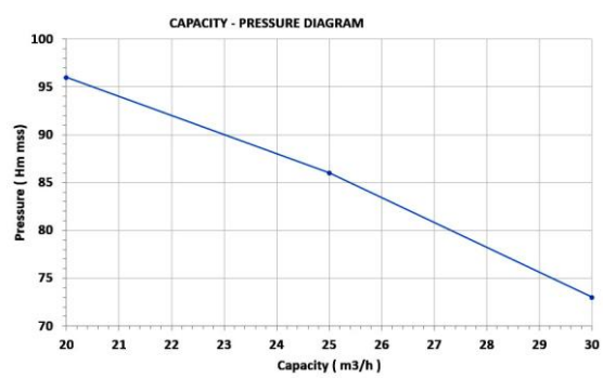
28,5 HP Lombardini Diesel Motopump - Electric Start
