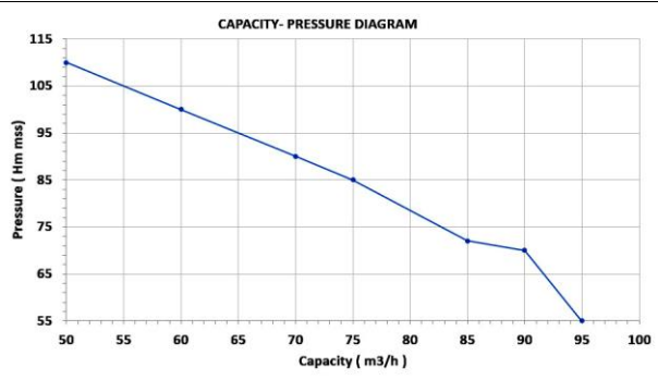
45 HP Diesel Motopump Water Cooler - 3 Stage With Trailer
