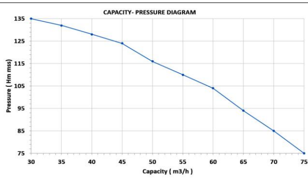
45 HP Diesel Motopump Water Cooler - 4 Stage With Trailer
